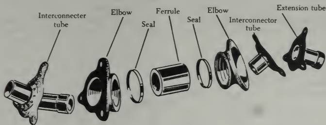
FIGURE 1-45. Interconnecting flame tubes for can-type combustion chambers.
